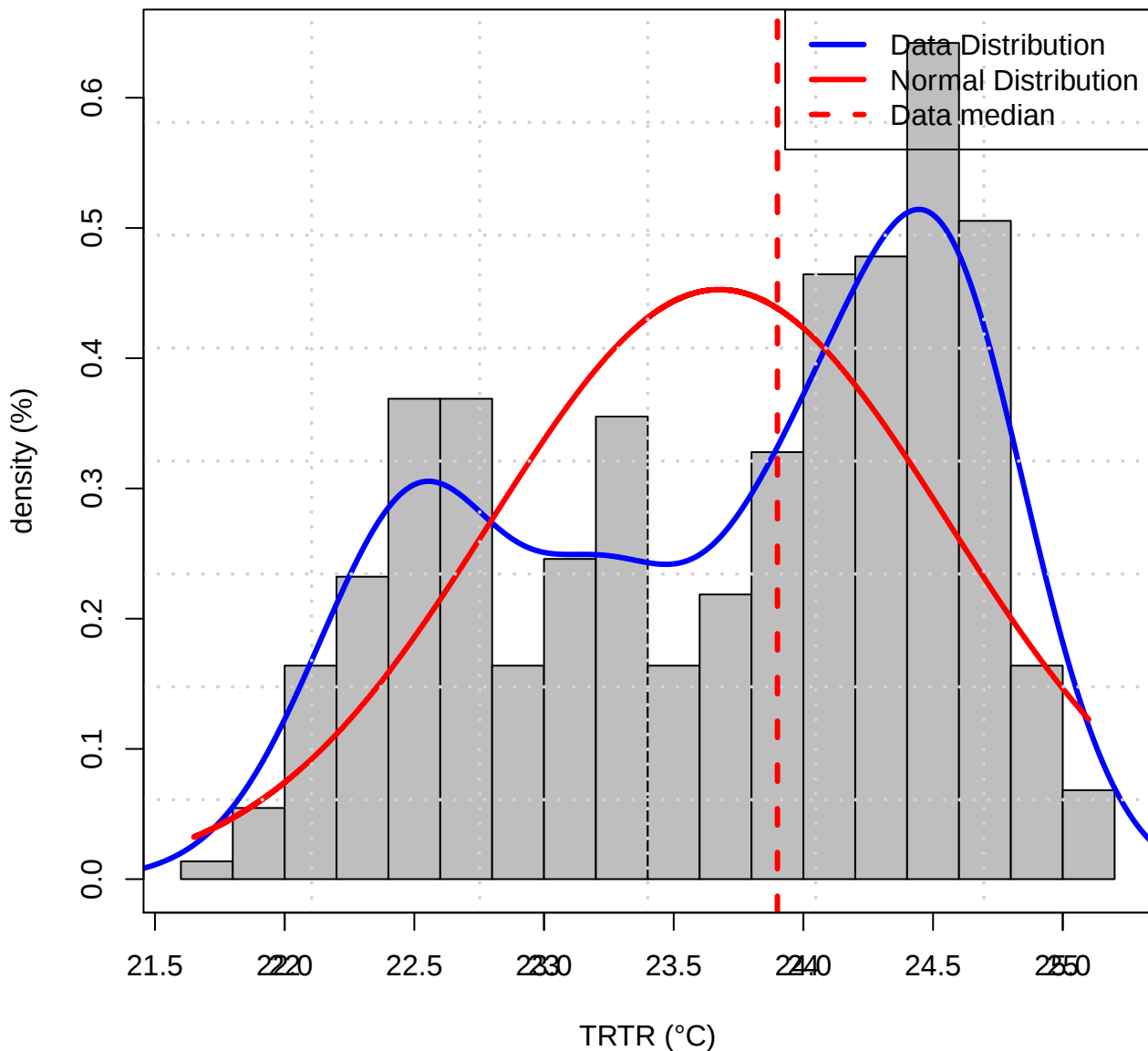
Histogram of Data distribution (TASMIN of TRTR)
