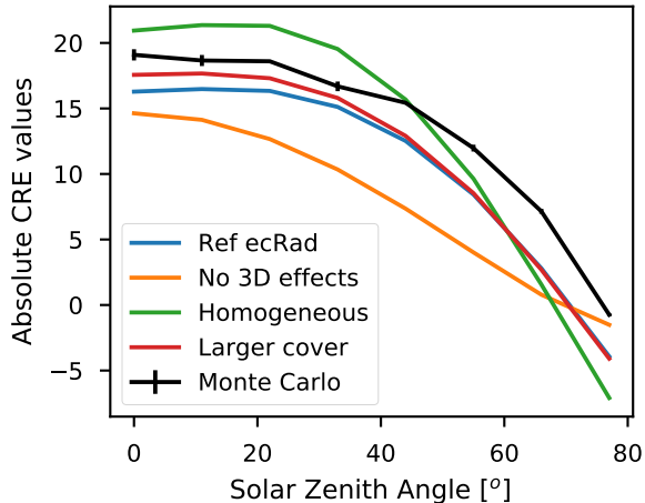
(a) CRE = total - clearsky [ \text{Wm}^{-2} ]
