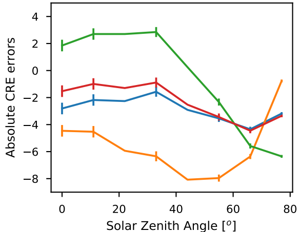
(b) \Delta \text{CRE} = \text{ecRad} - \text{MC} [ \text{Wm}^{-2} ]
