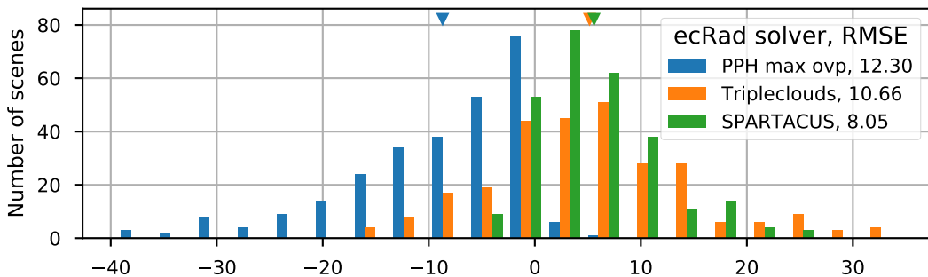
(b) Absorbed flux in the atmosphere
