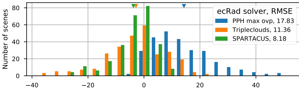
(c) Downward flux at surface
