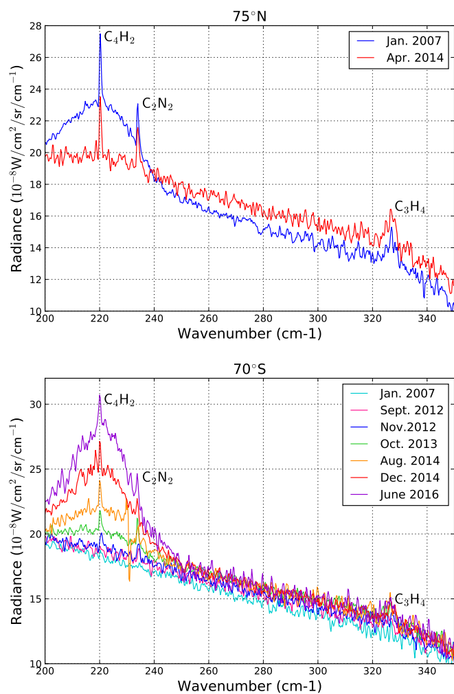
Fig. 8. Evolution of measured radiances at 75^\circ\text{N} (top panel) and 70^\circ\text{S} (bottom panel) from 2007 (northern winter) to 2016 (mid-spring). The sharp variation in the radiance between 228\text{ cm}^{-1} and 231\text{ cm}^{-1} in the spectra measured in August 2014 is a spurious noise feature which could not be eliminated during the calibration process. From 2007 to 2016, radiance at high southern latitudes has strongly increased, whereas it has decreased at high northern latitudes.
