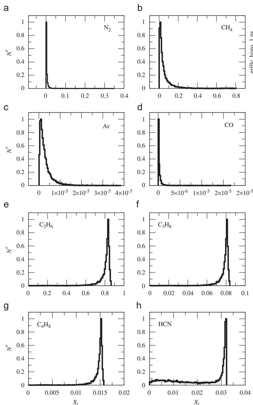
Fig. 1. (a–h) Histogram of mole fractions of Titan's hydrocarbon lakes. N^* is the normalized number of mole fractions owning the value X_i , computed within a given range of uncertainties for compound i (indicated in the top left of each panel). The 10,000 computations of chemical compositions have been performed at T=90 K, assuming a maximum error of \pm 10\% for all P_{vap} , V_m , \Delta H_m , and assuming a 0–0.1 range of values for the l_{ij} 's.
