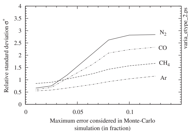
Fig. 3. Relative standard deviation \sigma_i^* corresponding to the mole fractions of N_2 , CH_4 , Ar and CO . \sigma_i^* are plotted as functions of the maximum errors obtained for P_{vap,i} , V_{m,i} , \delta H_{vap,i} in Monte Carlo simulations. l_{ij} 's have been set to 0.1 in all these computations.
