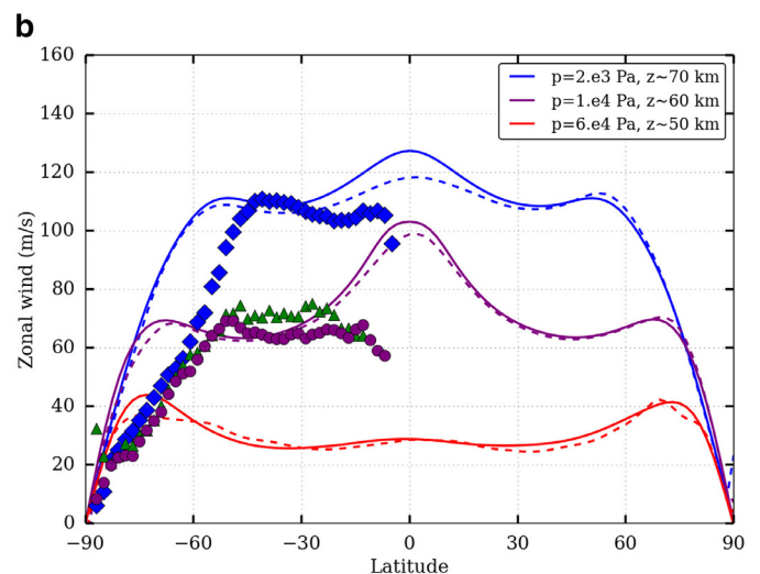
Fig. 6. Zonal and temporal averaged profiles of the zonal wind: (a) vertical profiles at three different latitudes, compared to observed profiles from Venera and Pioneer Venus probes (gray, adapted from Schubert, 1983 ); (b) latitudinal profiles at roughly 50, 60 and 70 km altitude, compared to averaged cloud-tracking zonal wind profiles obtained with VIRTIS-M images at UV (blue diamonds), visible (green triangles) and near-IR (magenta circles) wavelengths. They correspond to altitudes 66–72 km for UV spectral range, and a few kilometers below that level for visible/near-IR wavelengths (adapted from Hueso et al., 2015 ). The dashed lines are from the simulation started from rest, after 300 Vd. (For interpretation of the references to color in this figure legend, the reader is referred to the web version of this article.)
