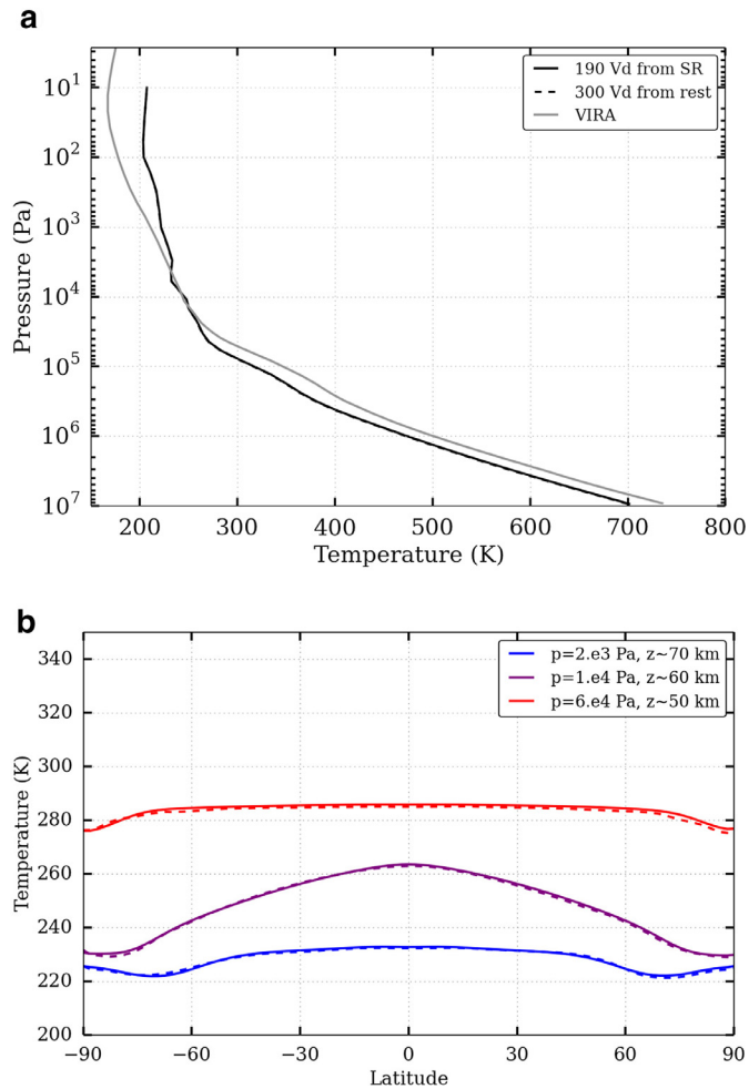
Fig. 1. Temperature structure obtained in the simulation started from superrotation, after 190 Vd: (a) vertical profile of globally averaged temperature; (b) latitudinal profiles of temperature (zonal and temporal average) at roughly 50, 60 and 70 km altitude. The dashed lines are from the simulation started from rest, after 300 Vd.
