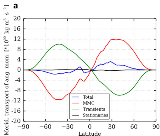
Fig. 10. Meridional (a) and vertical (b) transport of angular momentum, separating MMC contribution from transients and stationaries. The net horizontal transport is compensated by exchanges with the solid surface. However, the net vertical transport should be zero and the residual is indicative of the numerical inaccuracies discussed at the end of Section 2.1.
